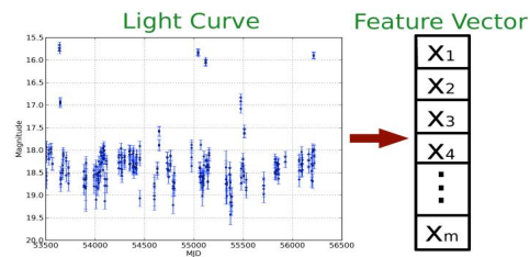
Fig. 2. Through the CTSCS a set of statistical descriptors are extracted from each light curve forming a feature vector. The plot shows a light curve of a Cataclysmic Variable from CRTS.
