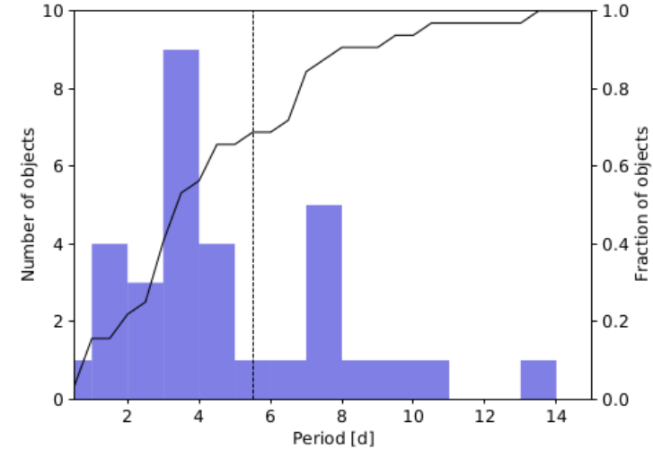
Figure 1. Distribution of measured periods of YSOs in our IC 5070 sample. The solid black line represents the cumulative distribution function. The dashed vertical line placed at a period of 5.5 d separates slow from fast rotators.
