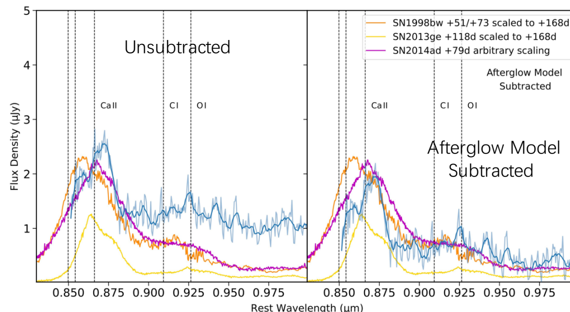
Spectrum(0.825-1 \mu\text{m} )
