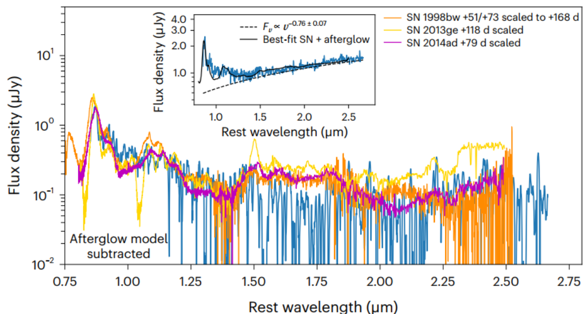
Afterglow model subtracted spectrum
